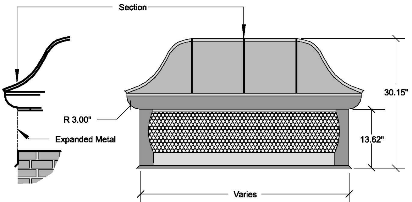
Side View
